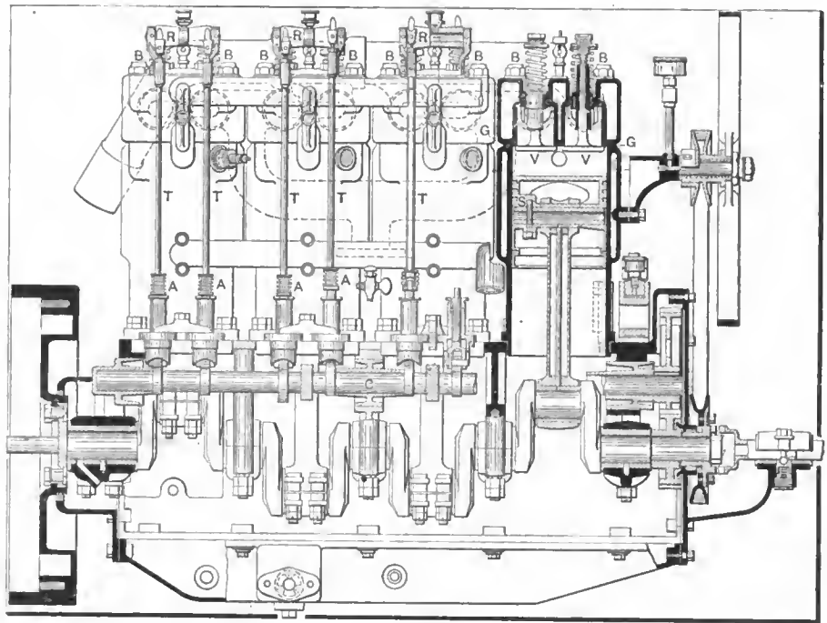
Fig. 2—View of the new Knox four-cylinder, long-stroke motor
